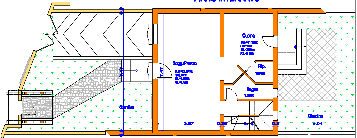
PIANO TERRA
