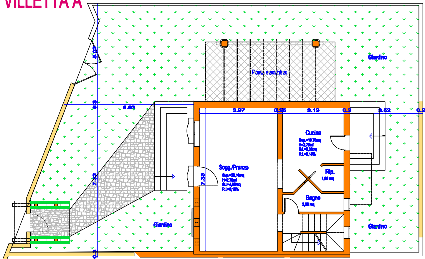
PIANO TERRA
